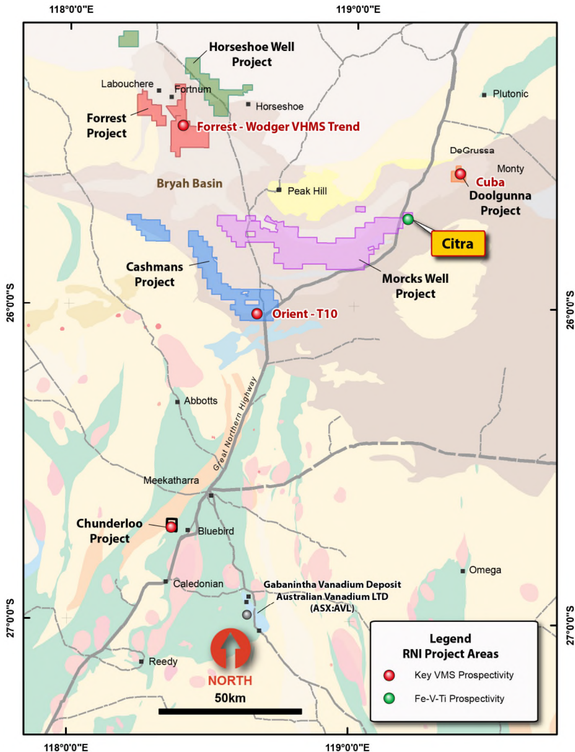
Figure 1: Citra V-Fe-Ti prospect in relation to RNI's existing land tenure
