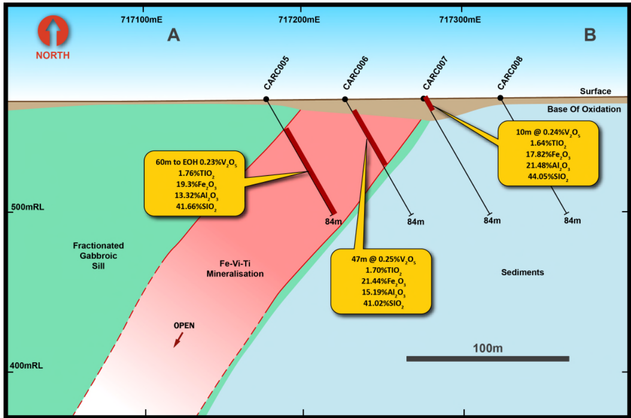
Figure 3: Cross section A-B showing anomalous V 2 O 5 , TiO 2 , Fe 2 O 3 , Al 2 O 3 and SiO 2 mineralisation – Citra Prospect
