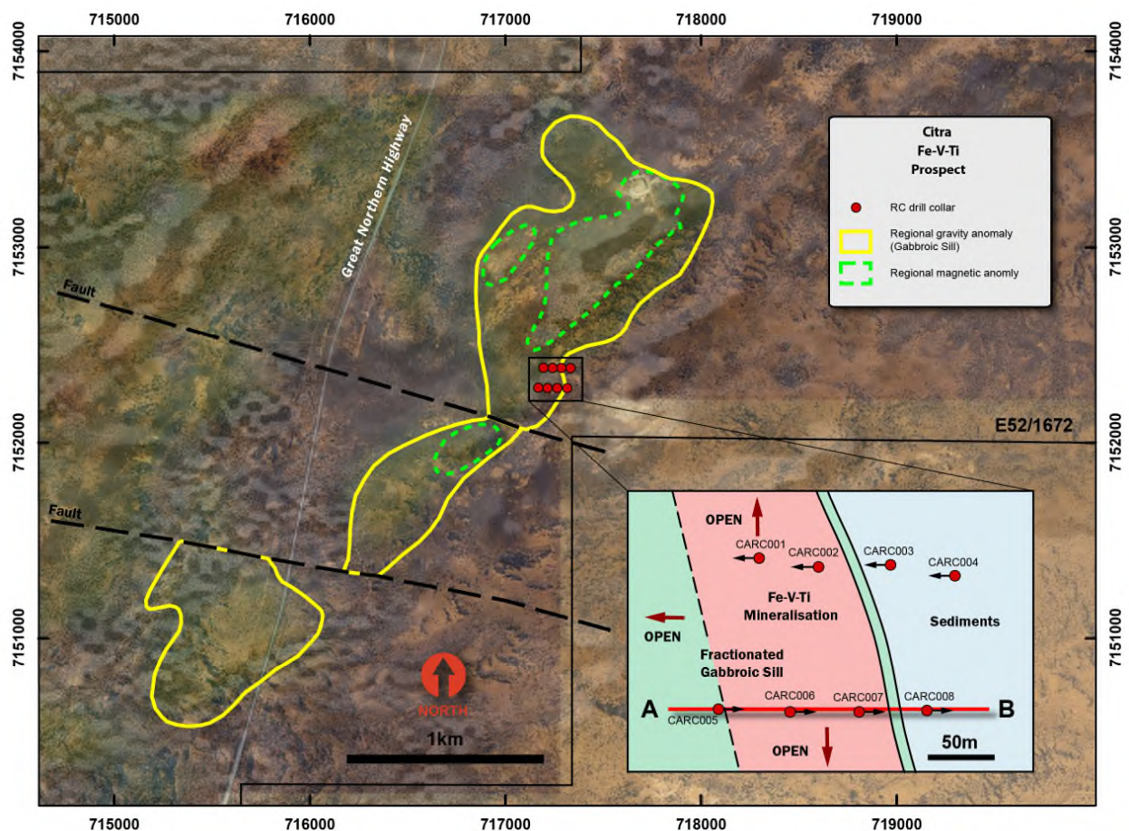
Figure 2: Topographic section showing existing RC drill collars in relation to known geophysical and geochemical anomalism – Topographic, 2VD magnetic and coloured gravity image underlay - Citra Prospect
