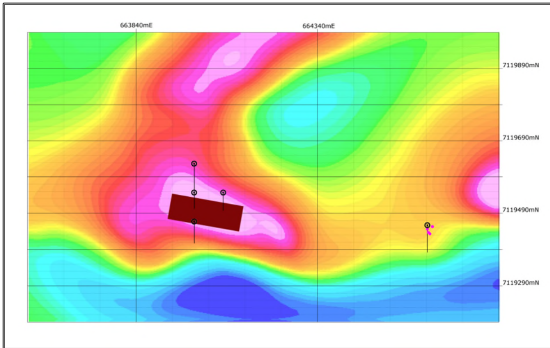
Figure 3: Plan view of the T10 target drilling and EM conductor plate modelling
